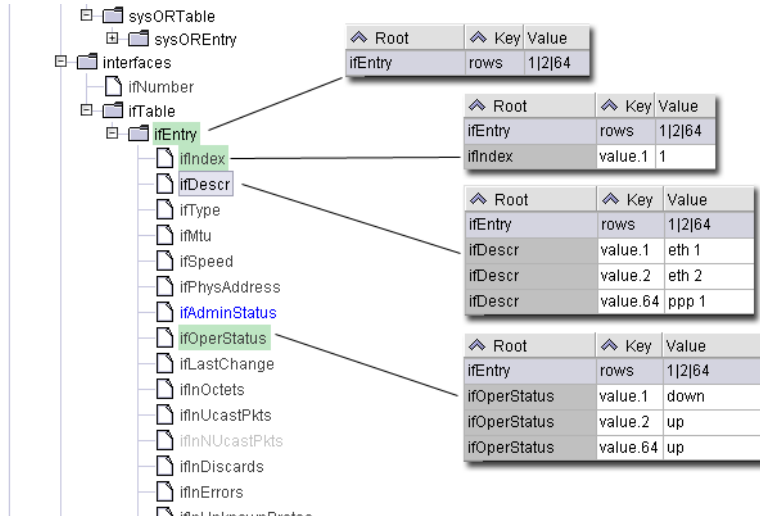
Figure 5: Example properties to simulate table data.
