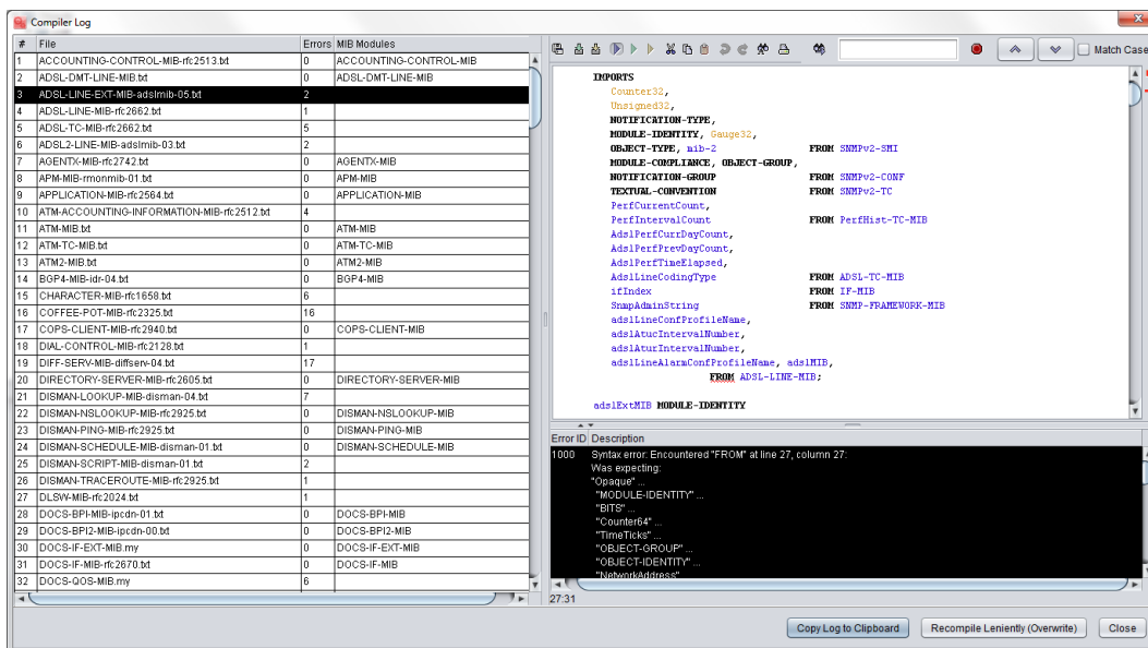
Figure 1: Compiler Log window with compilation errors displayed per MIB module.
