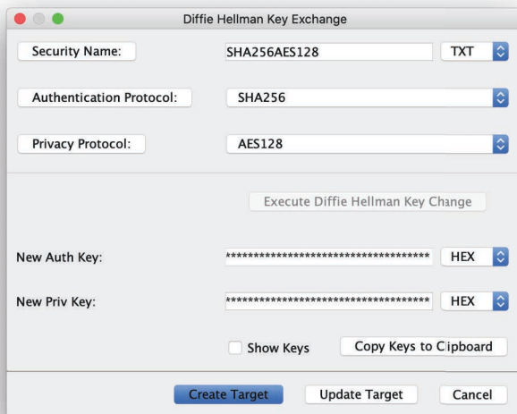
Figure 18: Diffie Hellman Key Exchange dialog
